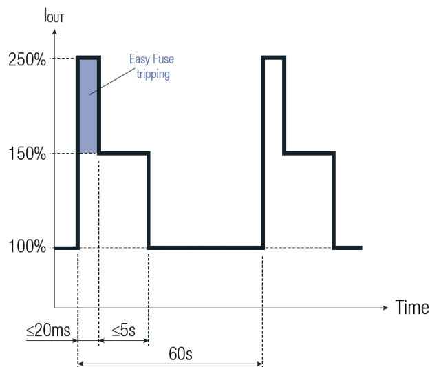
Boost Power (400V-480VAC or 500VDC; -40°C to +60°C max.)
