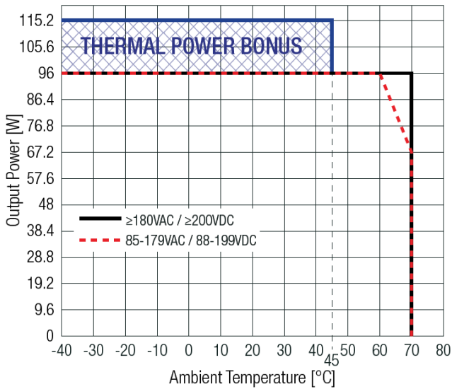
Derating Graph (@ Chamber and natural convection 0.1m/s, standard mounting orientation)
