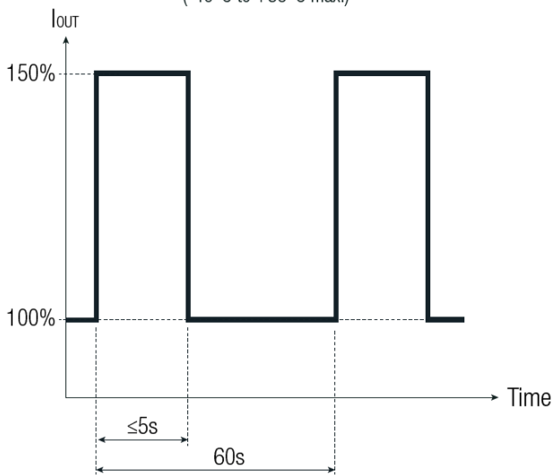
Boost Power (-40°C to +60°C max.)
