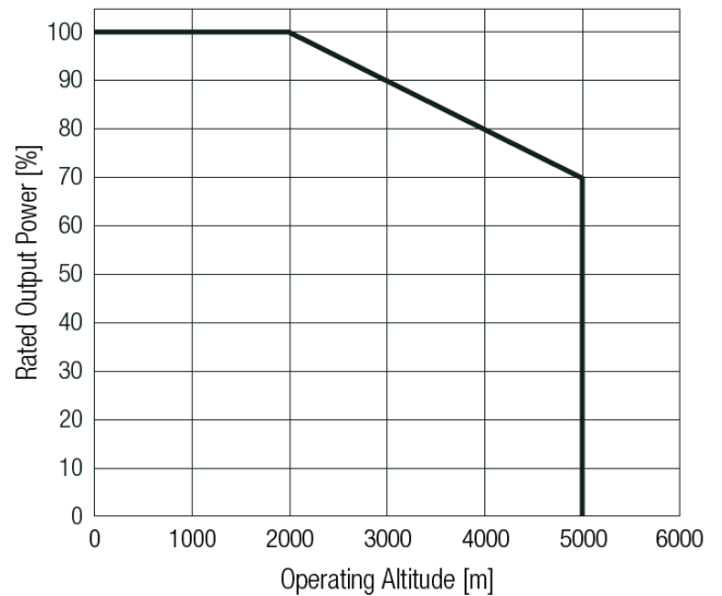
Altitude Derating
