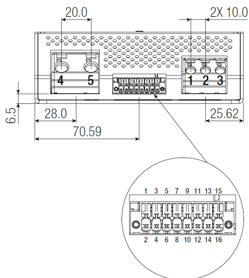
Input connector CAGE CLAMP® CON1 (WAGO 745-353)
