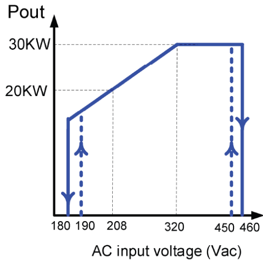
Mode 1: AC-DC charging mode
