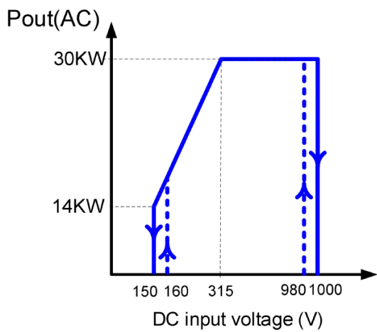
Mode 2: Grid forming mode, AC voltage output
