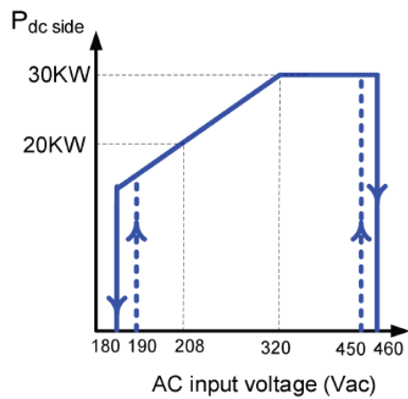
Mode 3: Grid connection mode, P/Q control
