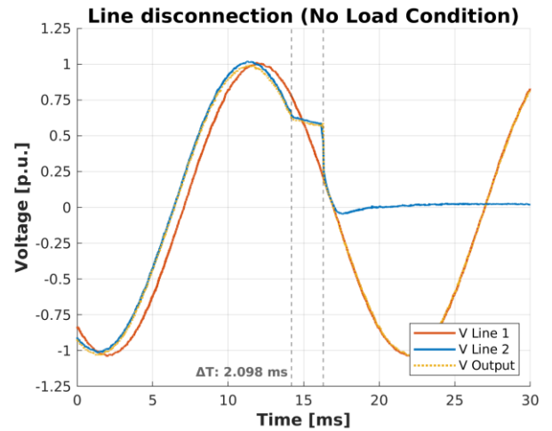
Example of line disconnection at no load condition (<20W).
