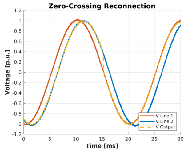
Example of reconnection to the priority line.
