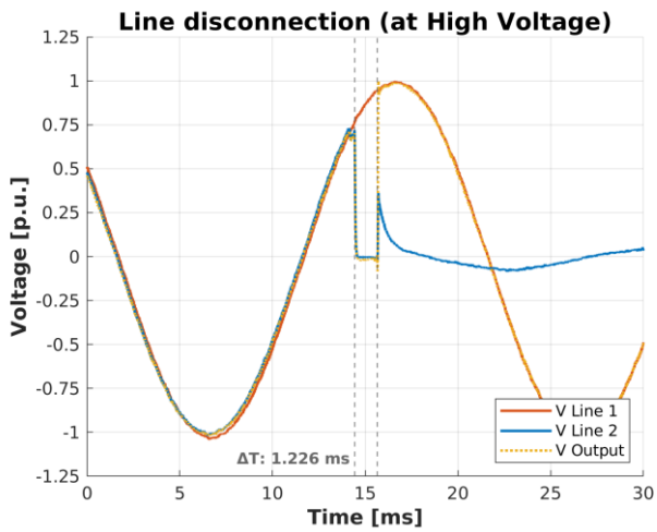
Example of line disconnection. Line fault at high voltage.
