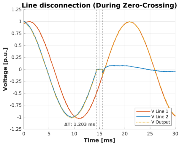
Example of line disconnection. Line fault at 0V.
